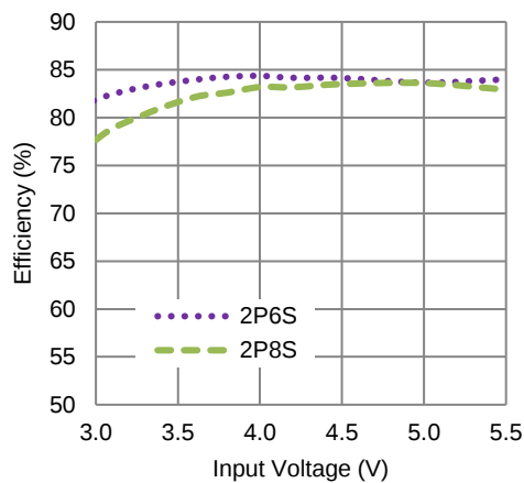
Efficiency vs. Input Voltage ( I_{OUT} = 40mA , 2P6S LEDs)
