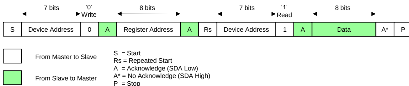
Figure 5. I 2 C Read Cycle
