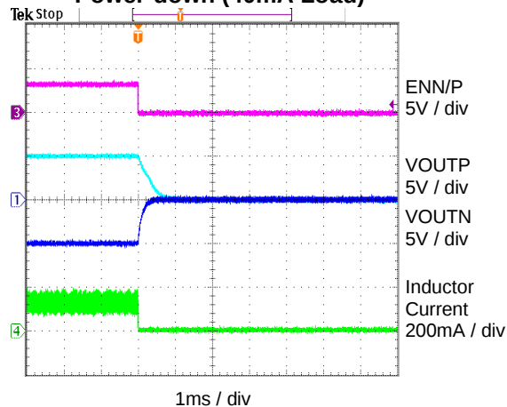
Power-down (40mA Load)
