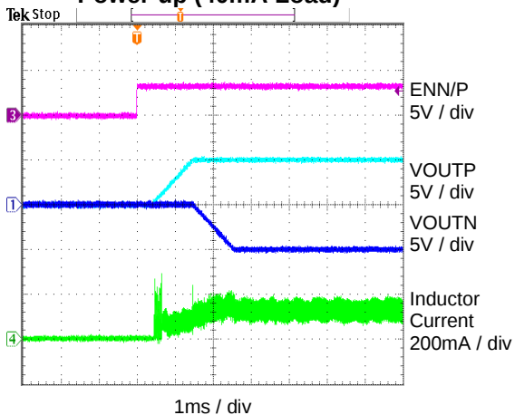
Power-up (40mA Load)
