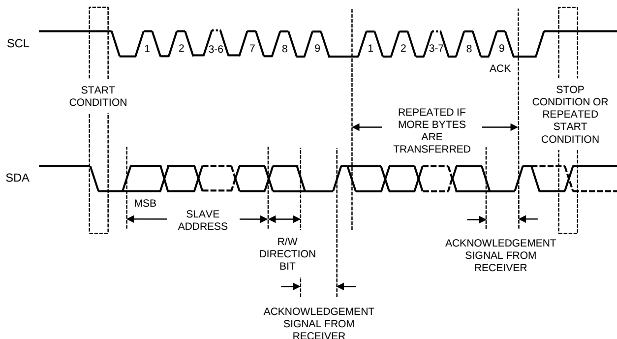
Figure 3. Data Transfer on I2C Serial Bus
