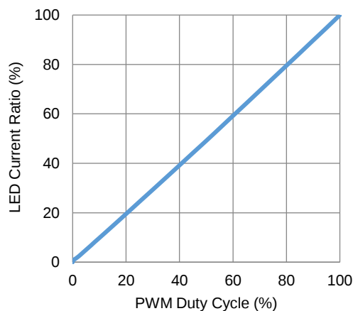
PWM Dimming Linearity (20kHz)
