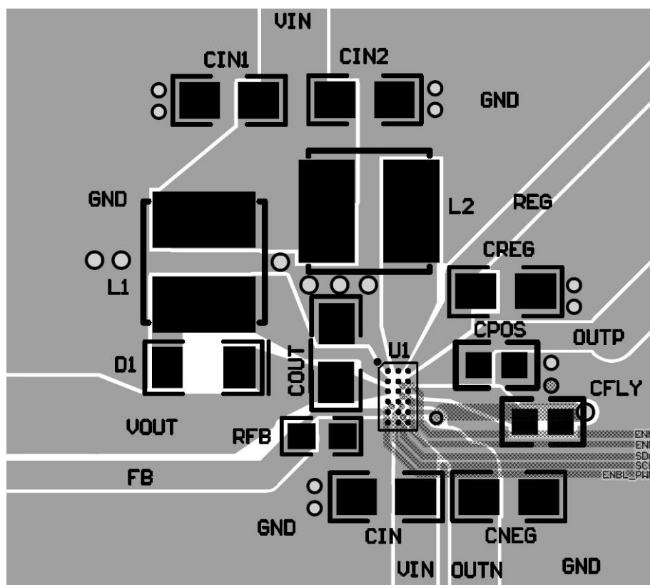
Figure 6. Recommended PCB Layout
