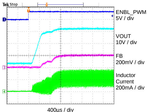
Turn On with LED Open (OVP)
