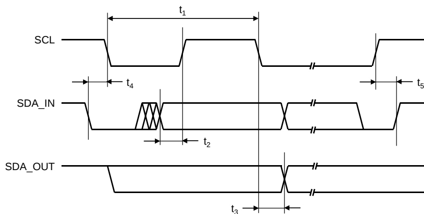
Figure 2. I 2 C Compatible Interface Timing
