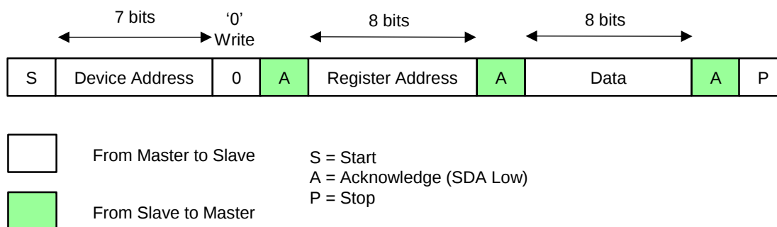
Figure 4. I 2 C Write Cycle
